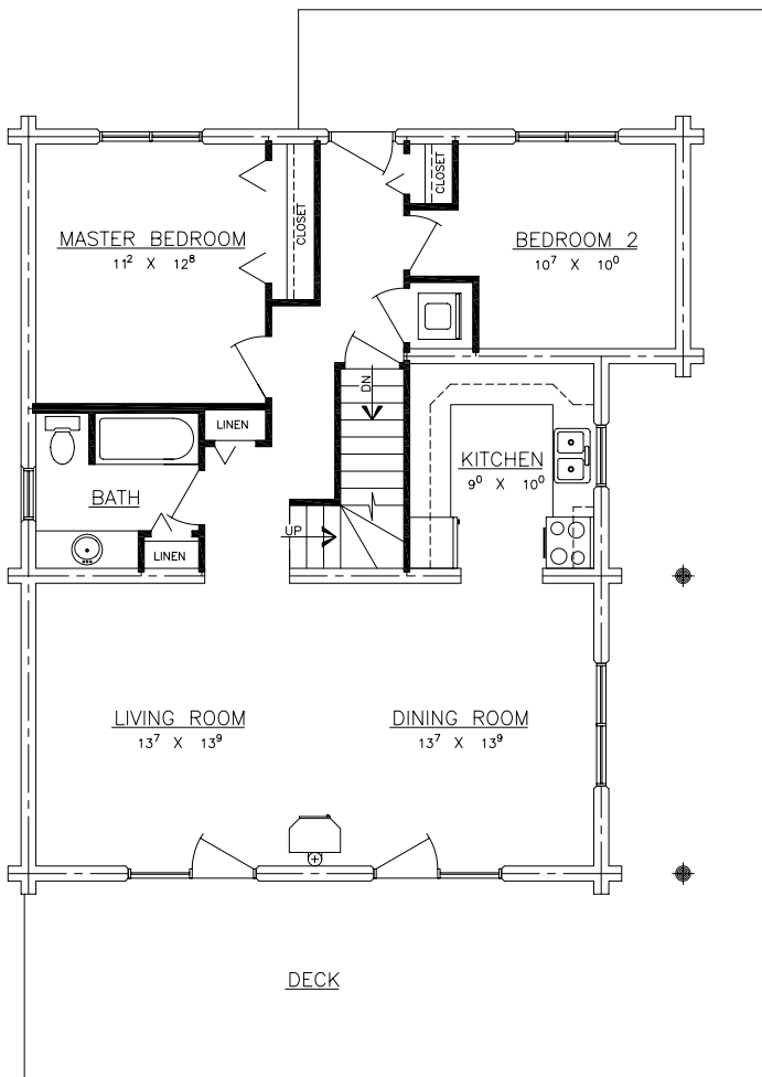
MAIN FLOOR AREA = 1051 S.F.
