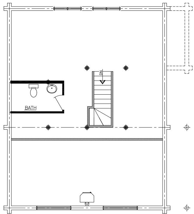
SECOND FLOOR AREA = 622 S.F.
